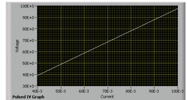
Figure 5b: Pulsed I-V curve over the same range.
